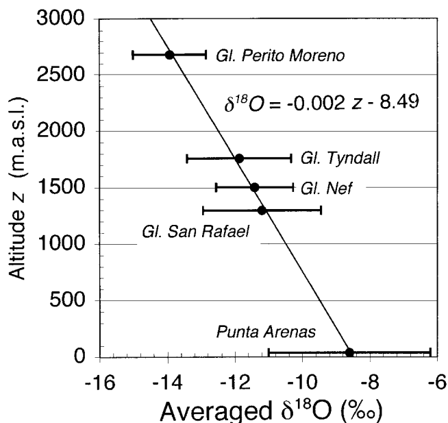
Fig. 4. Relationship between averaged values of \delta^{18}\text{O} and altitudes in the two Patagonia icefields and the nearest meteorological station. Original data for Glaciar San Rafael are from Yamada (1987); for Glaciar Perito Moreno from Aristarain and Delmas (1993); and for Glaciar Nef from Matsuoka and Naruse (1999). Data for Punta Arenas were obtained from the GNIP database ( http://www.iaea.org/programs/ri/gnip/gnipmain.htm ). Solid dots and bars are the average value and the standard deviation of each dataset used for analyses. See text for further explanation.
